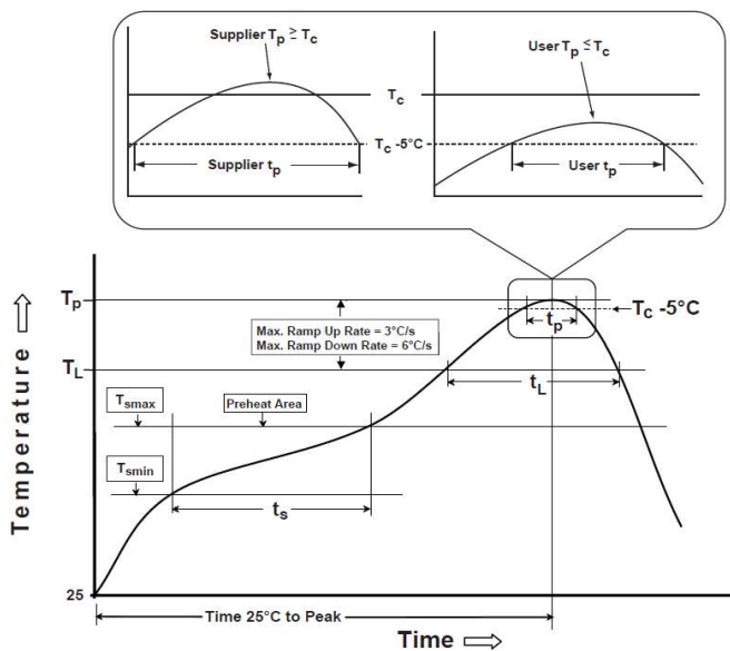
Fig.1 Soldering Reflow
